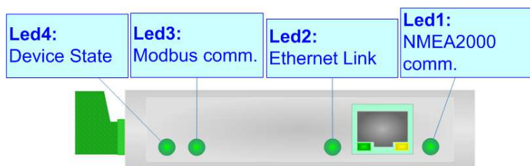
Led2: Green Ethernet Link
