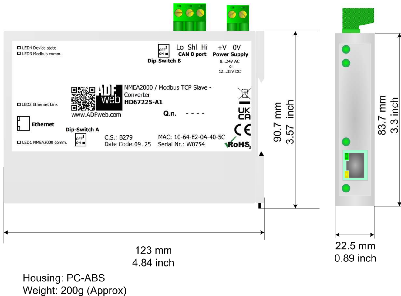
Figure 10a: Mechanical dimensions scheme for HD67225-A1
