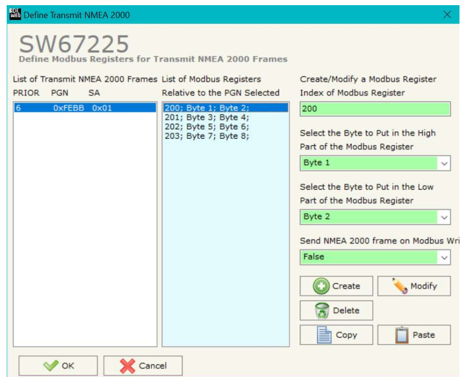
Figure 7: "Define NMEA 2000" window
