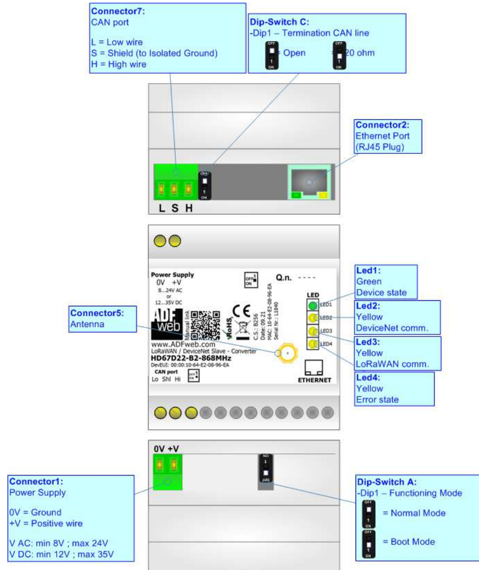
Figure 1: Connection scheme for HD67D22-B2-xxxMHz
