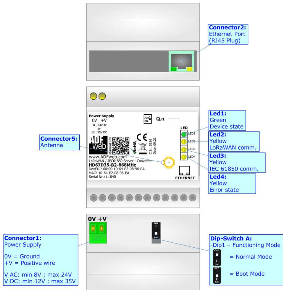
Figure 1: Connection scheme for HD67D35-B2-xxxMHz
