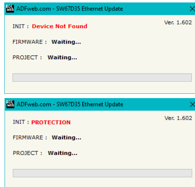
Figure 8: "Error" window
