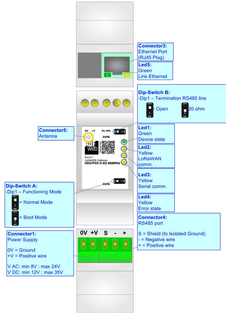
Figure 1b: Connection scheme for HD67F05-5-B2-xxxMHz
