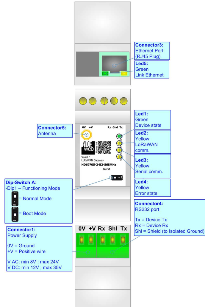
Figure 1a: Connection scheme for HD67F05-2-B2-xxxMHz
