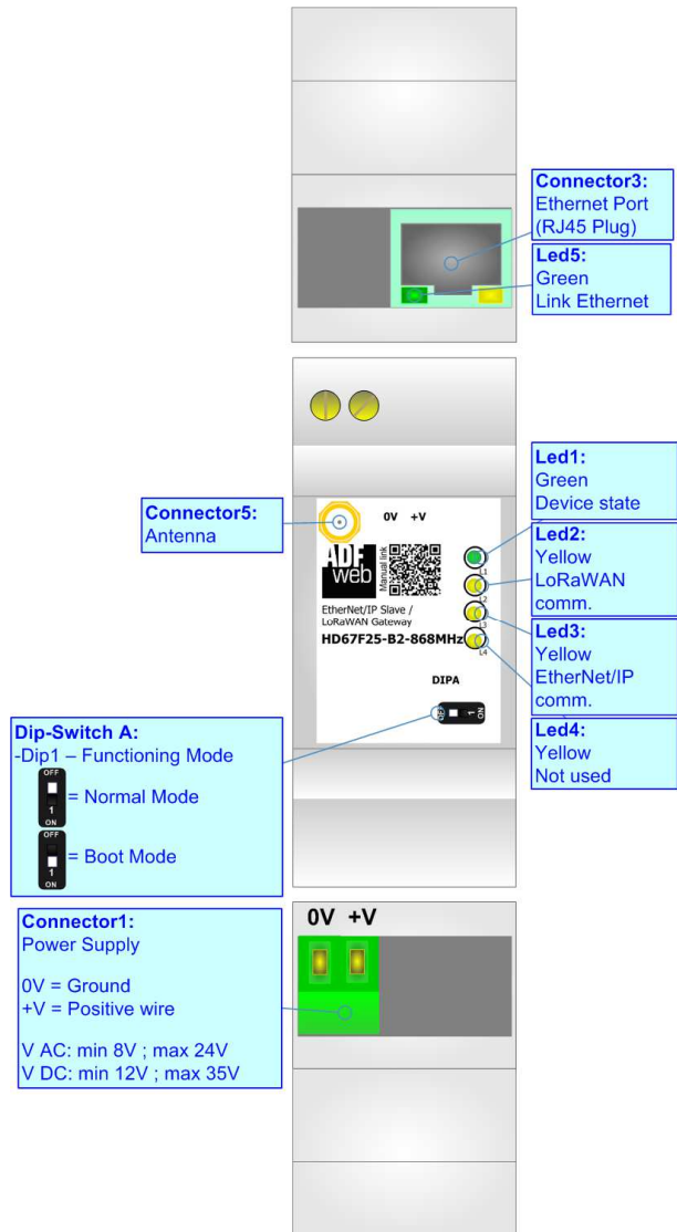
Figure 1: Connection scheme for HD67F25-B2-xxxMHz
